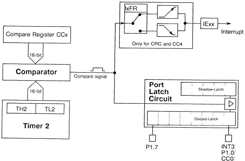
Figure 7-43 Timer 2 with Registers CCx (= CRC and CC1 to CC4) in Compare Mode 1
