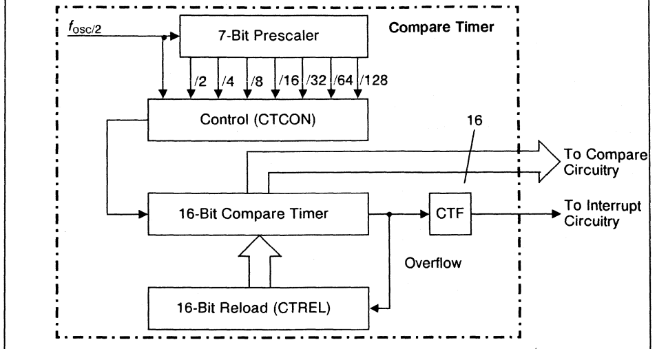
Figure 7 Block Diagram of the Compare Timer
