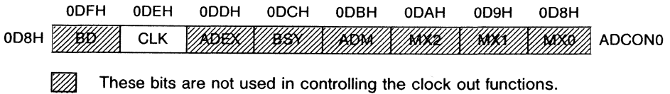
Figure 7-68 Special Function Register ADCON0 (Address 0D8H)
