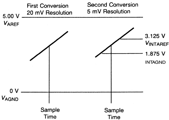
Figure 7-31 Increasing the Resolution by a Second Conversion
