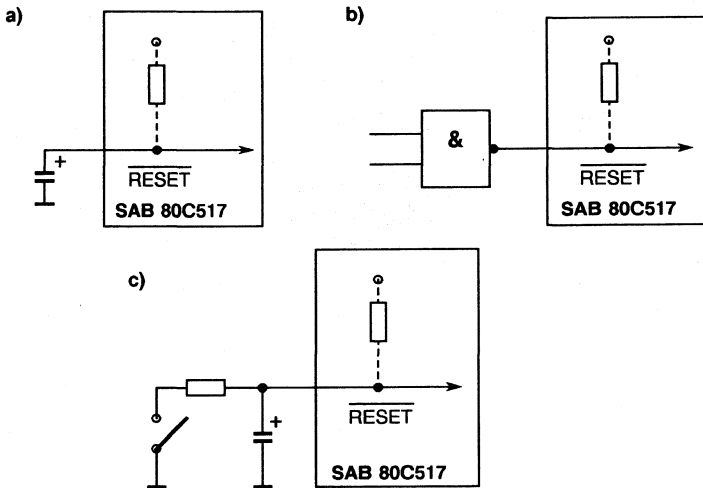
Figure 6-1 Reset Circuitries
