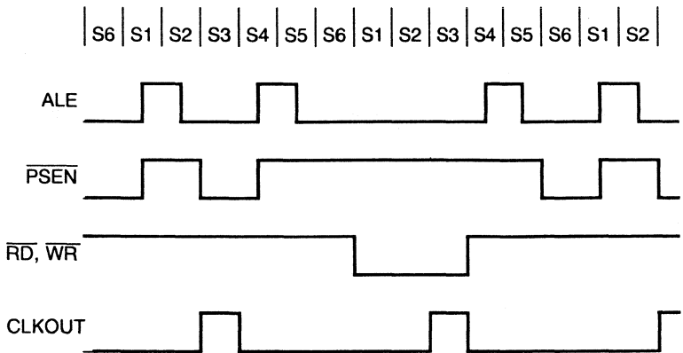
Figure 7-69 Timing Diagram - System Clock Output
