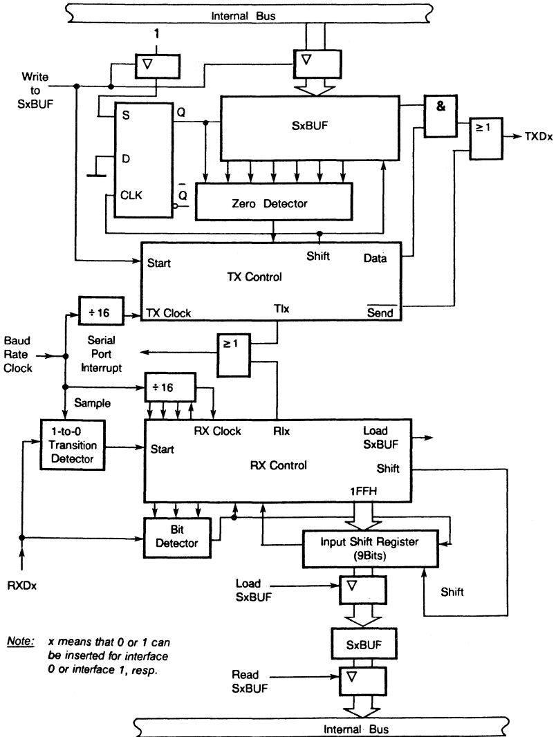
Figure 7-17 a) Functional Diagram - Serial Interfaces 0 and 1, Mode 1/Mode B
