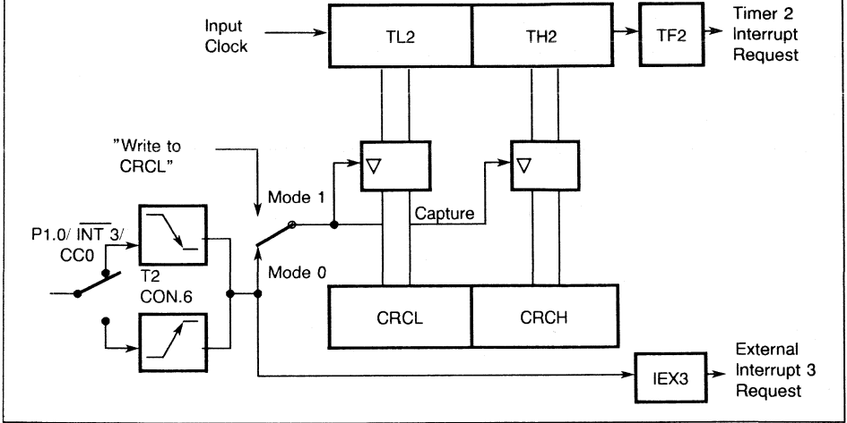
Figure 7-53 Capture with Registers CRC, CC4
