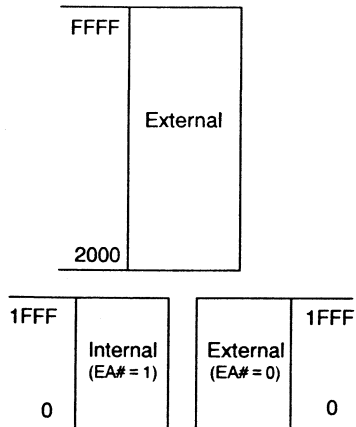
Figure 4-1 Program Memory Address Space
