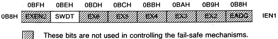
Figure 7-61 Special Function Register IEN1
