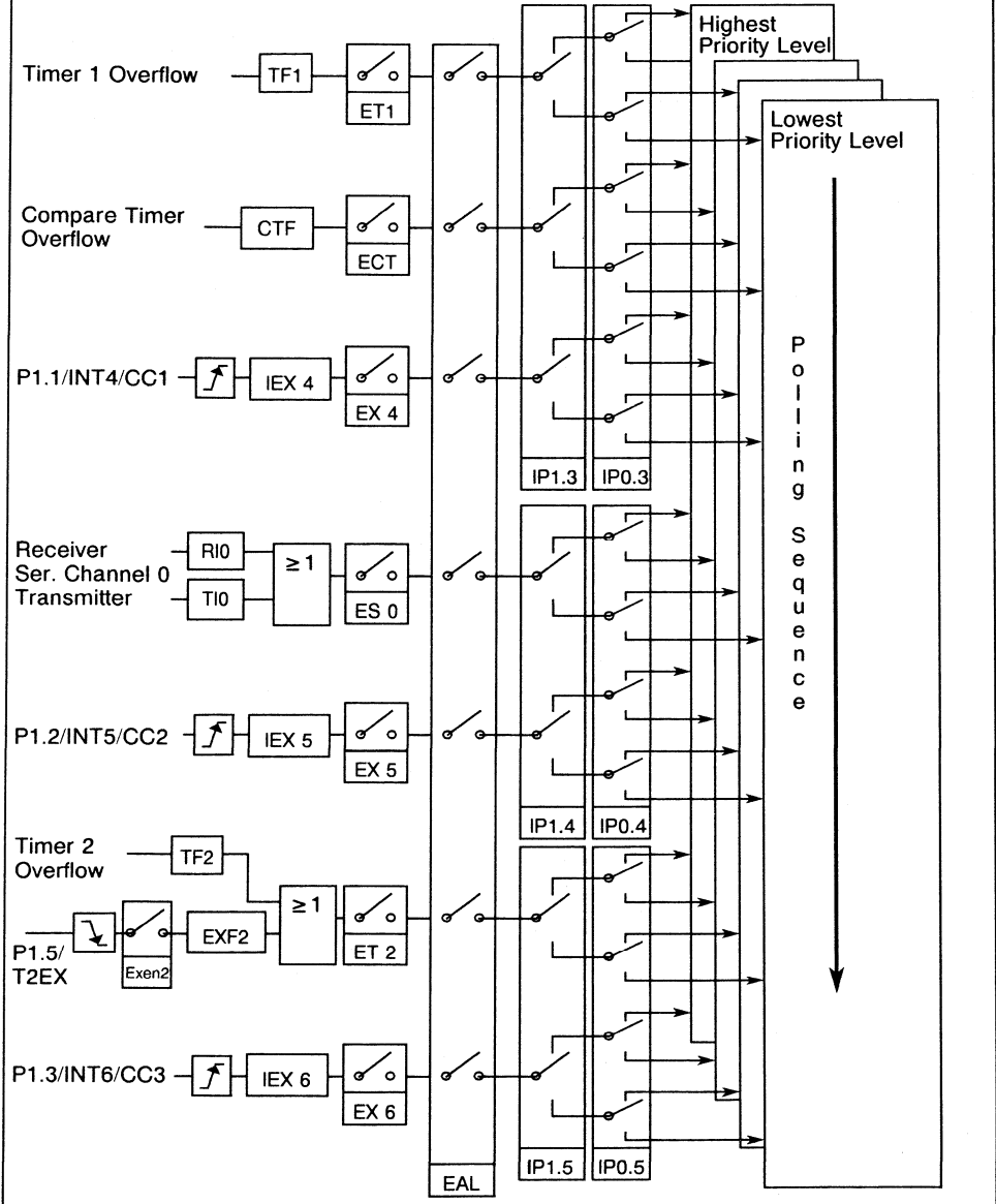
Figure 9 (cont'd) Interrupt Structure of the SAB 80C517
