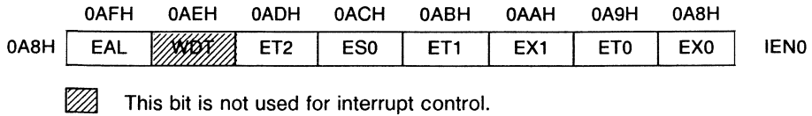
Figure 8-2 Special Function Register IEN0 (Address 0A8H)
