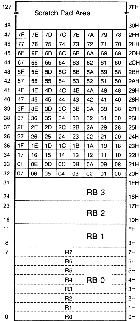
Figure 4-3 Mapping of the Lower Portion of the Internal Data Memory
