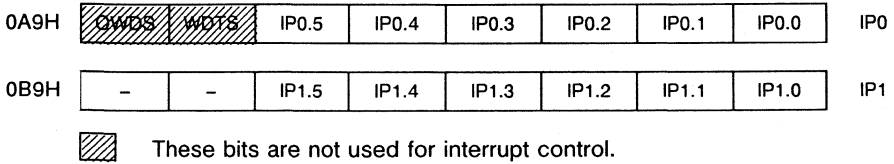
Figure 8-9 Special Function Registers IP0 and IP1 (Address 0A9H and 0B9H)
