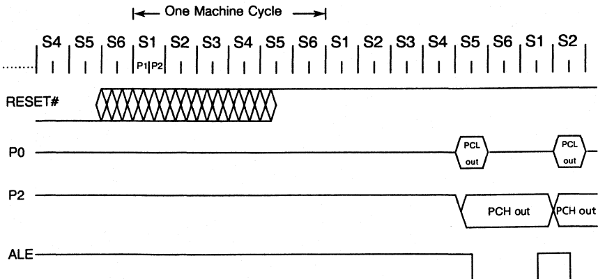
Figure 6-2 CPU Timing after RESET
