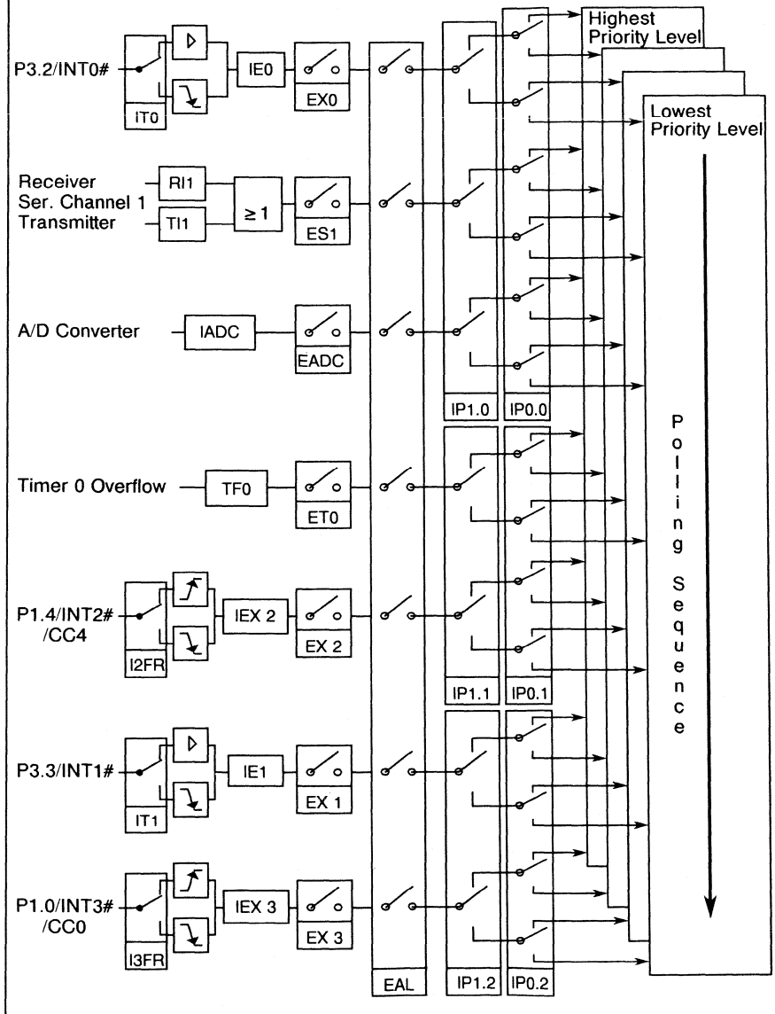
Figure 9 Interrupt Structure of the SAB 80C517
