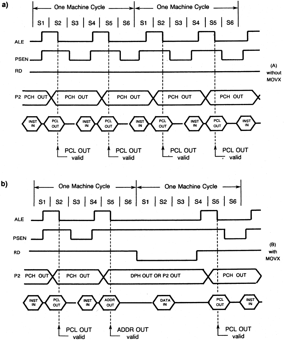
Figure 5-2 a) and b) External Program Memory Execution
