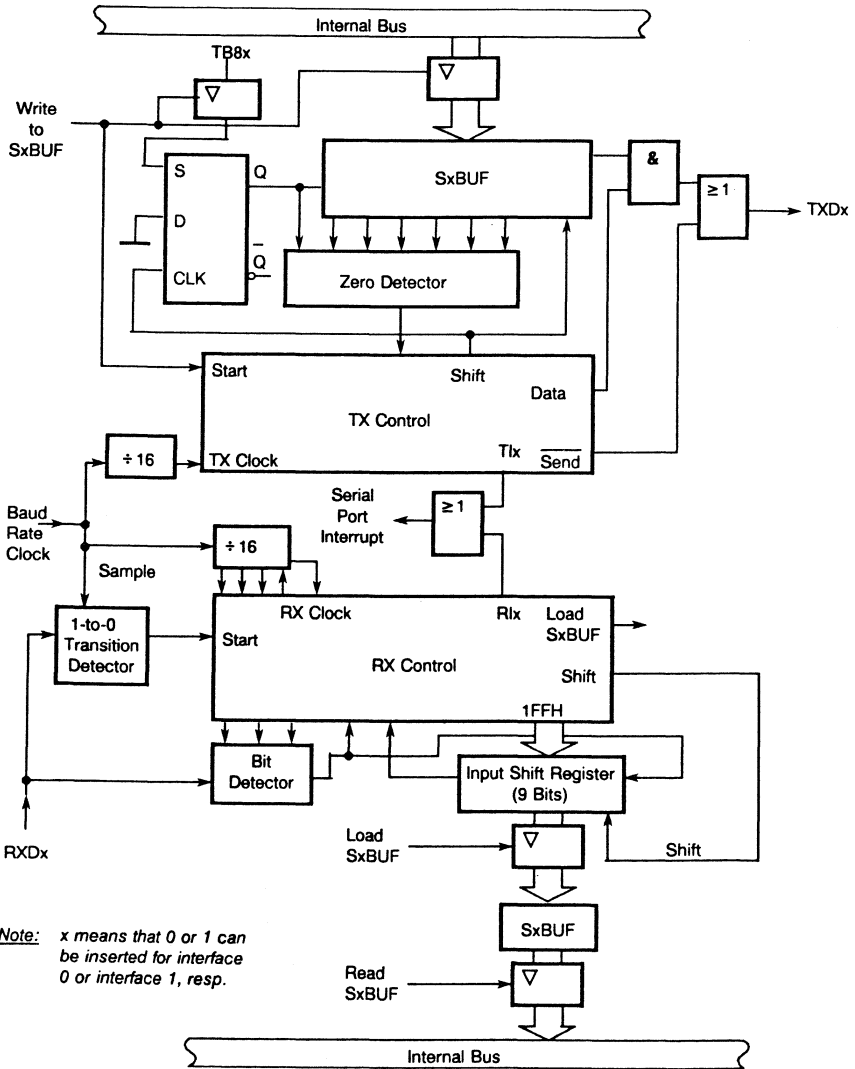
Figure 7-18 a) Functional Diagram - Serial Interface 0 and 1, Modes 2 and 3/Mode A
