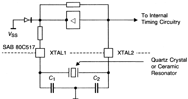
Figure 7-66 On-Chip Oscillator Circuitry
