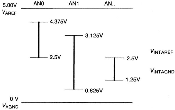
Figure 7-30 Adjusting the Internal Reference Voltages to the Range of the External Analog Input Voltages
