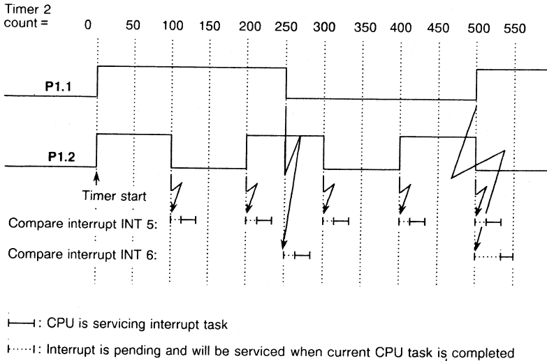
Figure 10-1 Task Schedule for "Additive Compare" Program
