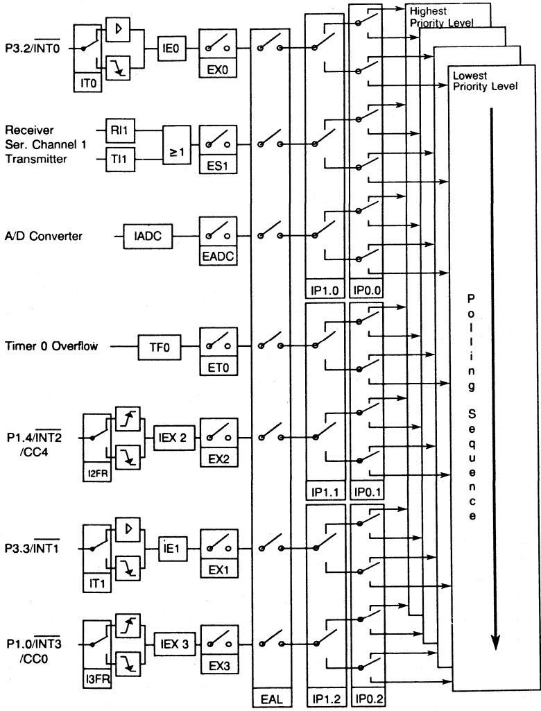
Figure 8-1 a) Interrupt Structure of the SAB 80C517
