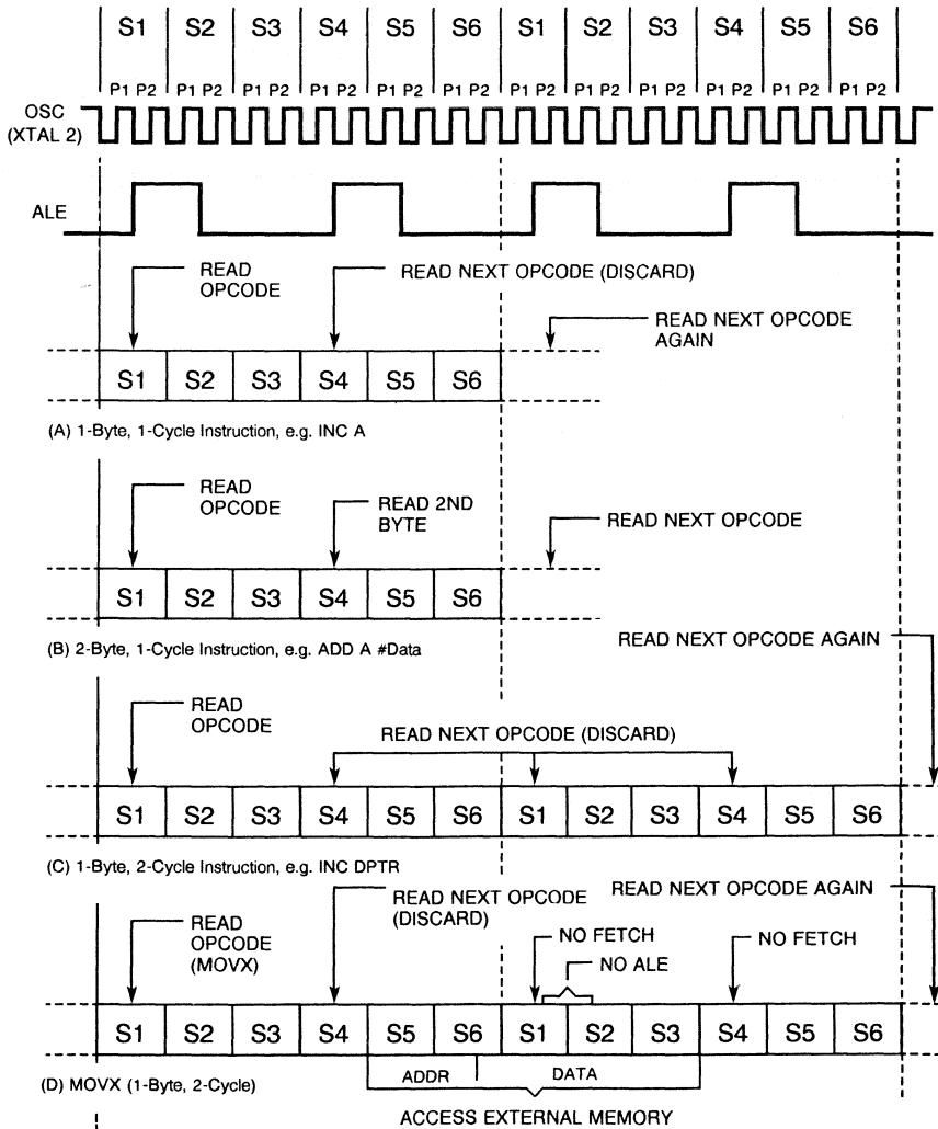
Figure 3-1 Fetch/Execute Sequence
