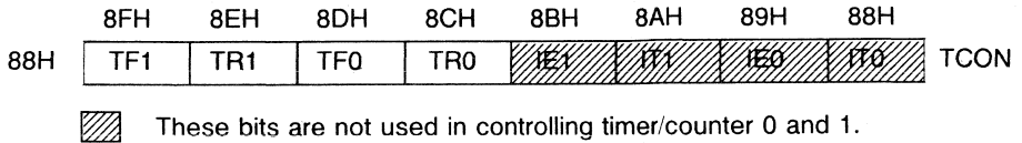
Figure 7-19 Special Function Register TCON (Address 88H)
