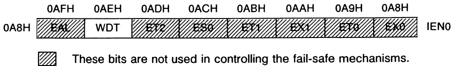
Figure 7-60 Special Function Register IEN0
