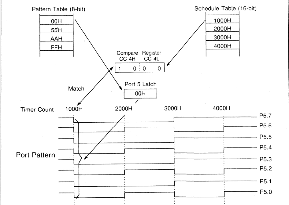
Figure 7-46 Example for a "Concurrent Compare" at Port 5
