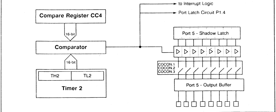
Figure 7-45 "Concurrent Compare" Function of Register CC4
