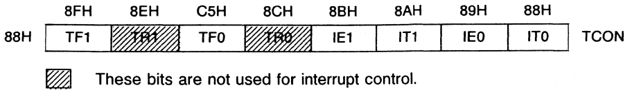
Figure 8-5 Special Function Register TCON (Address 88H)
