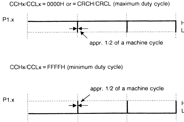
Figure 7-44 Modulation Range of a PWM Signal Generated with a Timer 2/CCx Register Combination in Compare Mode 0
