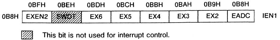
Figure 8-3 Special Function Register IEN1 (Address 0B8H)
